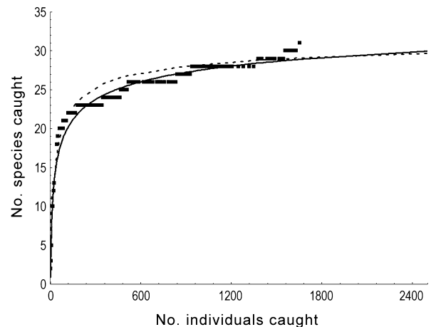
Fig. 6. Actual data and the species accumulation curve (Beta-P model) for Great Victoria Desert L area showing the increase in number of species caught late in the trapping program, and how the shape of the species accumulation curve differs depending on which data are used to calculate the curve (see text for explanation). (—), Predicted species accumulation curve based on all data points; (■), actual data points; (- - -), predicted species accumulation based on data points when a new species is caught.
